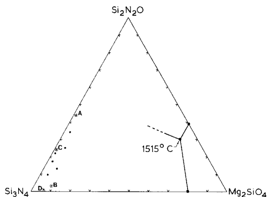
Figure 1 The \text{Si}_3\text{N}_4 - \text{Mg}_2\text{SiO}_4 - \text{Si}_2\text{N}_2\text{O} system illustrating compositions of materials used in this study in relation to eutectic composition.
